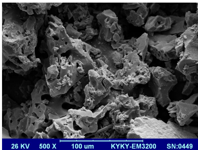
FIGURE 1 The SEM image of NiFe 2 O 4 nano catalyst
